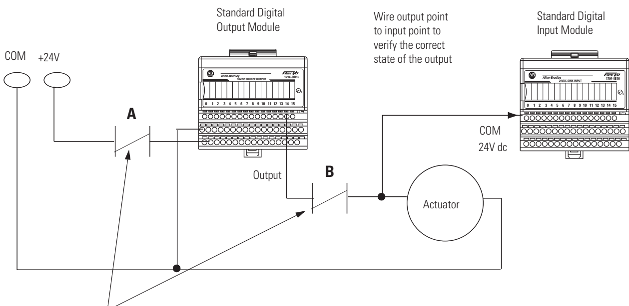
Figure 3.5 ControlLogix/FLEX I/O Standard Output Module Wiring
