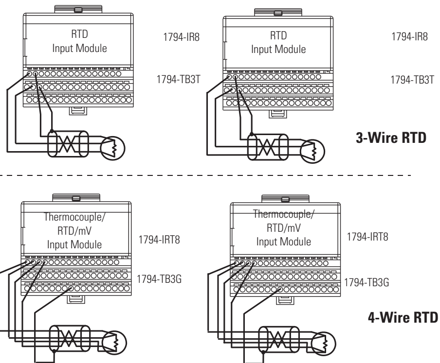
Figure 3.11 FLEX I/O Analog RTD Module Wiring
